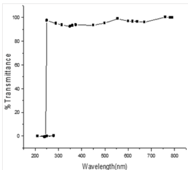
Figure 9: Graph 150 °C annealed CuO sample
