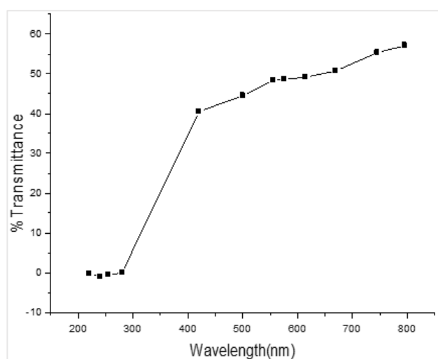
Figure 10: Figure 8: Graph 200 °C annealed CuO sample
