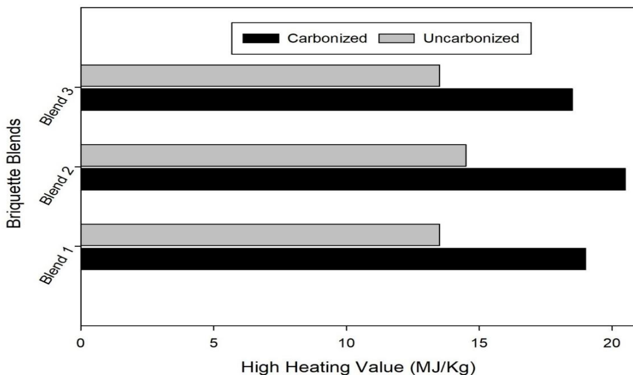
Figure 2: Higher heating values of Carbonized and uncarbonized Briquettes
