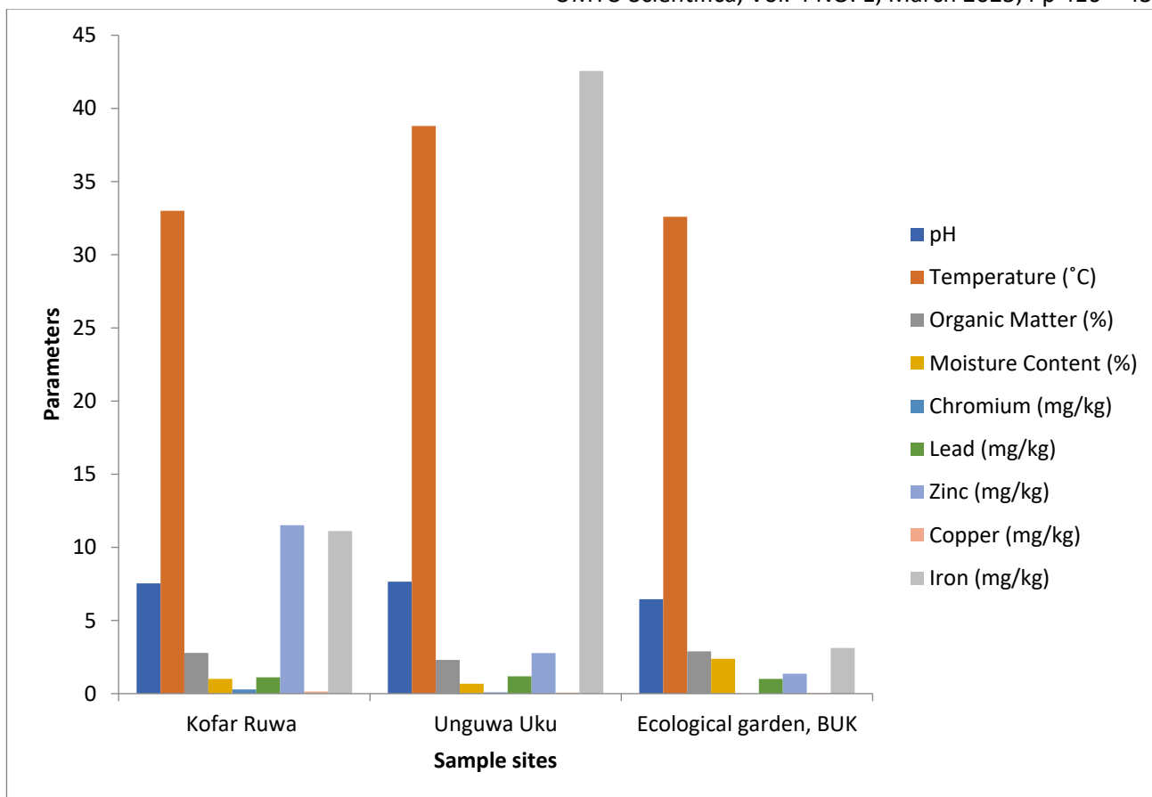
Figure 1: Physico-chemical properties of the soil samples at Kofar Ruwa, Unguwa Uku, and Ecological garden BUK.
