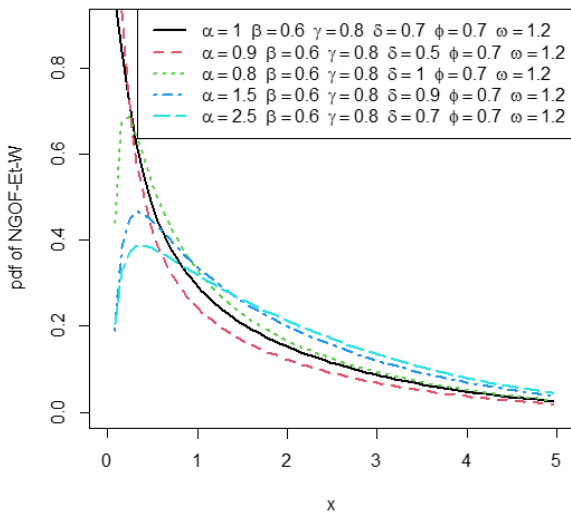
Figure 3: PDF Plot of New Generalized Odd Frechet-Exponentiated-Weibull Distribution
