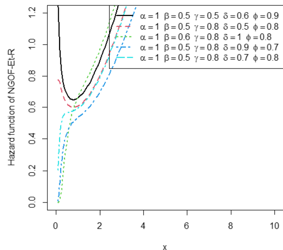
Figure 2: Hazard Plot of New Generalized Odd Frechet Exponentiated-Rayleigh Distribution
