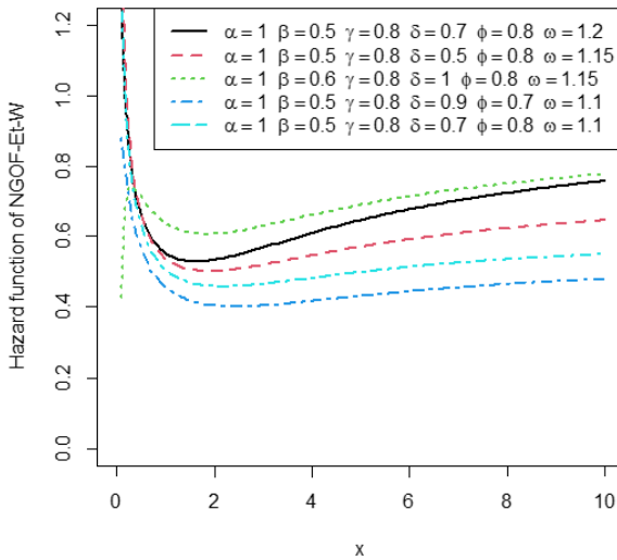
Figure 4: Hazard Plot of New Generalized Odd Frechet-Exponentiated-Weibull Distribution
