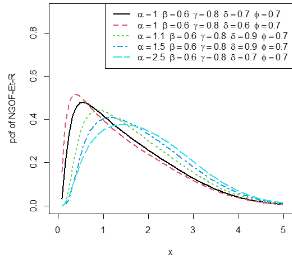
Figure 1: PDF Plot of New Generalized Odd Frechet Exponentiated-Rayleigh Distribution
