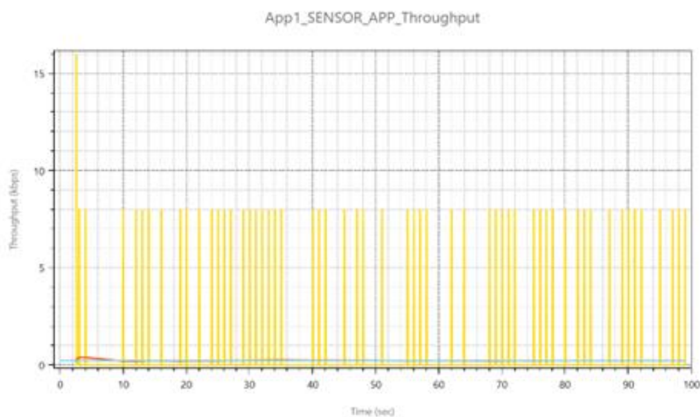
Figure 2: security threat
