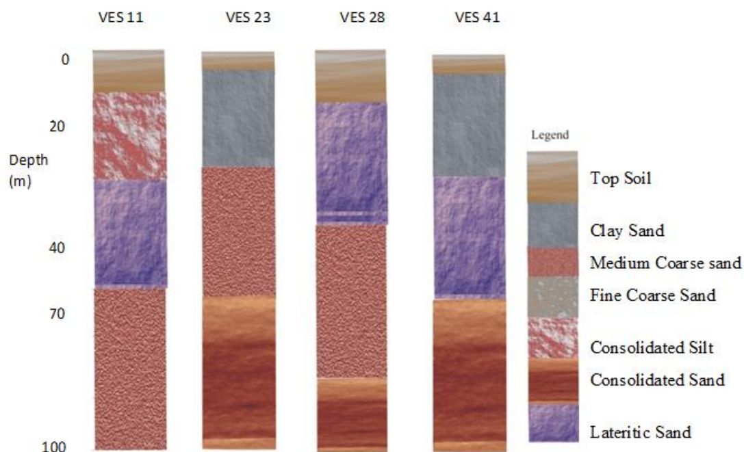
Figure 5: Lithologic section.
