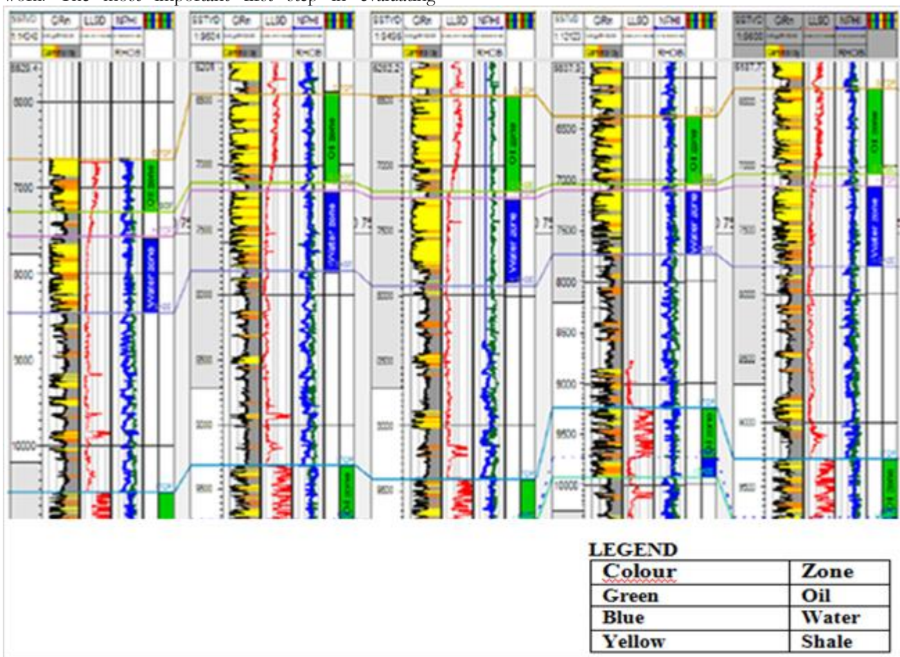
Figure 2: Geophysical well log Obtained from the Petrel and OpendTect Software
