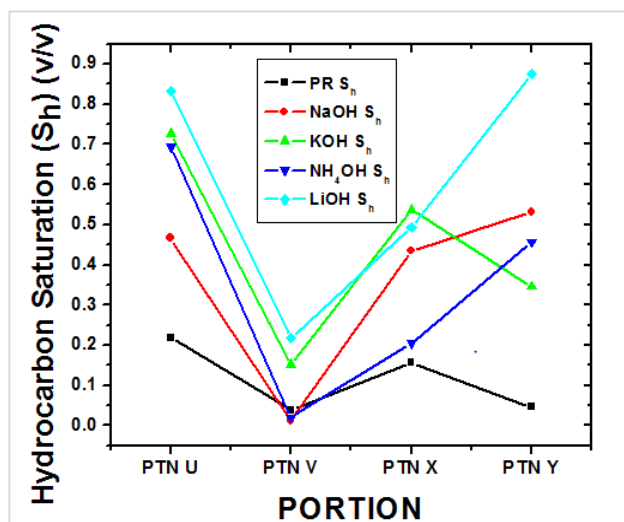
Figure 6: Comparison of the PR S_h and the EOR S_h
