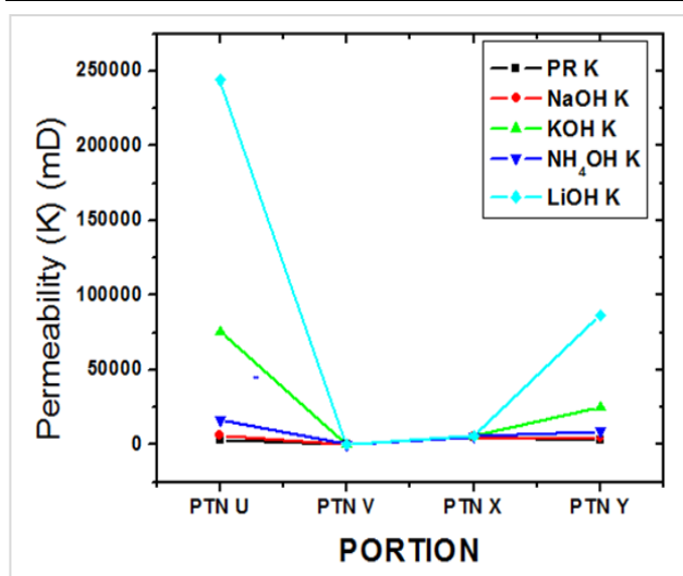
Figure 4: Comparison of the PR K and the EOR K
