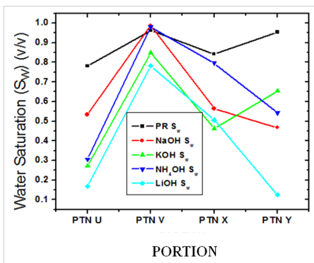
Figure 5: Comparison of the PR S_w and the EOR S_w
