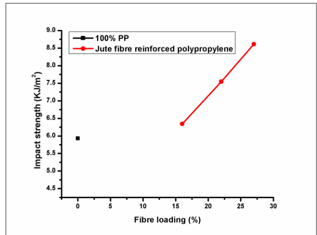
Figure 3.5: Impact strength VS Fibre loading.
