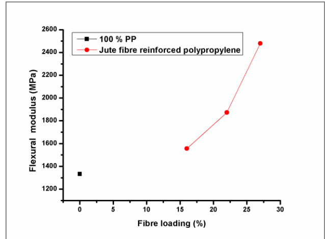
Figure 3.4: Flexural modulus VS Fibre loading.
