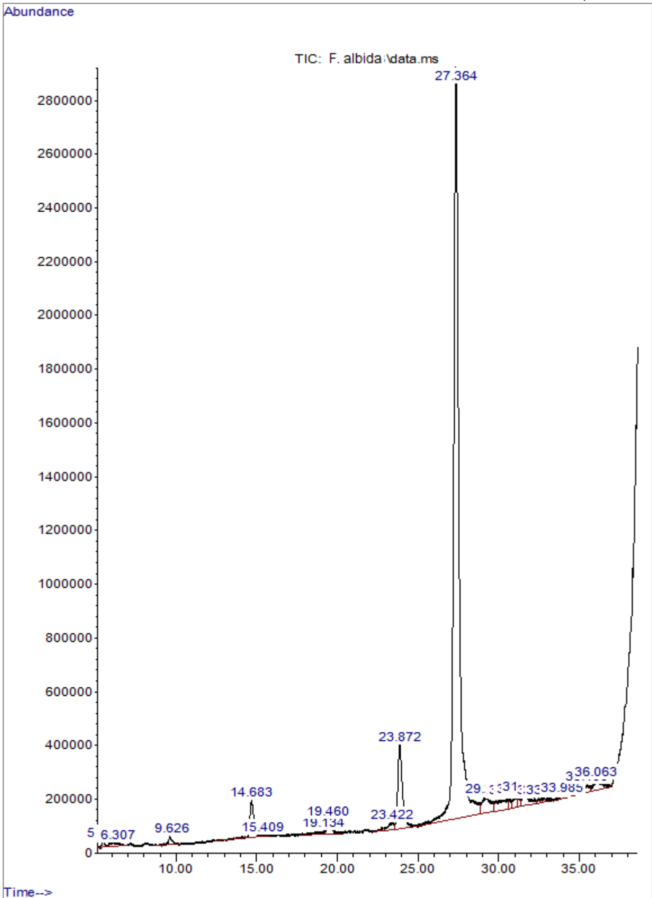
Figure 6: GC-MS chromatogram ethanolic extract of Faidherbia albida leaf
