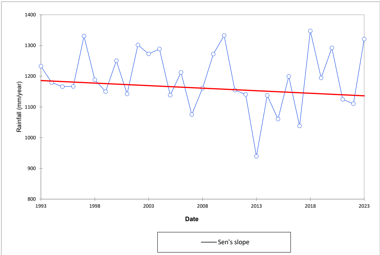
Figure 6a: Mann-Kendall trend test: Annual Rainfall
