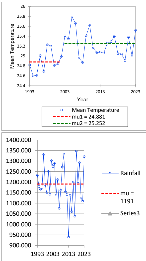
Figure 2: PT and SNHT Homogeneity tests for mean temperature and rainfall; (up) Mean temperature (down) Rainfall
