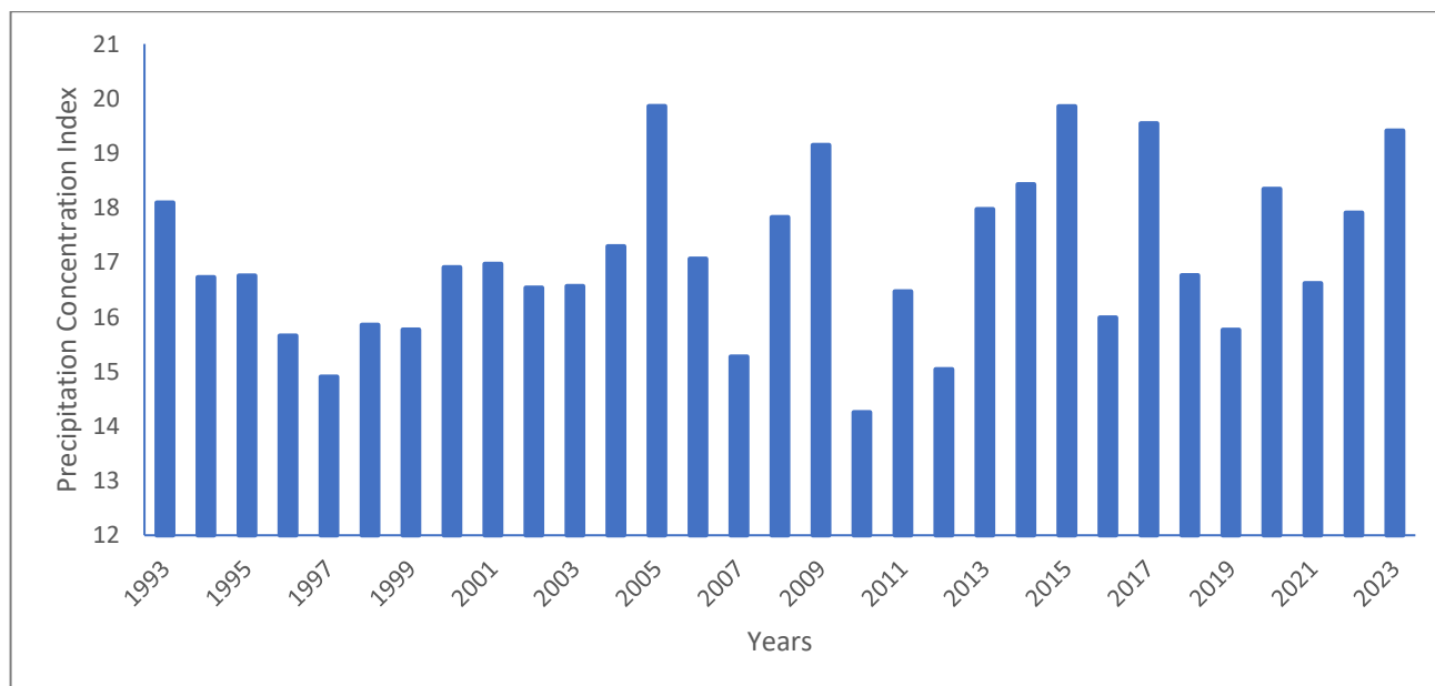
Figure 5: Precipitation Concentration Index in Kaduna North LGA
