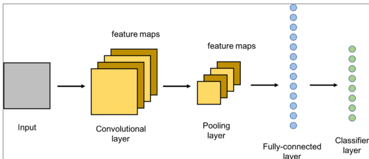
Figure 2: Typical CNN Model Architecture (Adopted from Zaniolo et al., 2020 )
